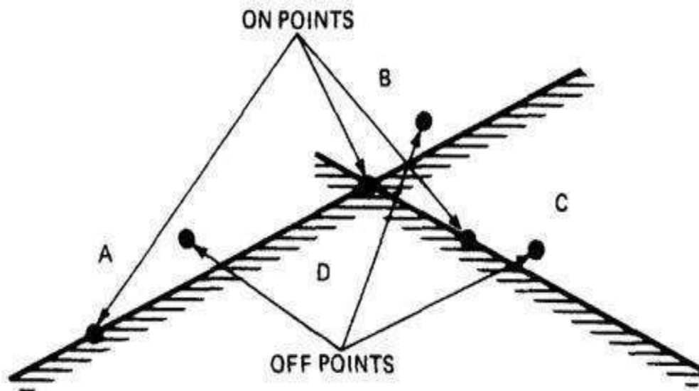
Figure 4.11: On points and Off points.
