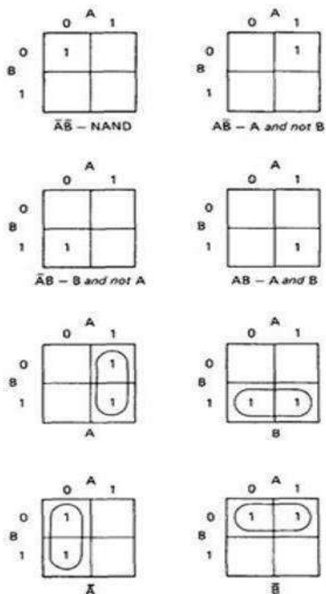
Figure 6.7: KV Charts for Functions of Two Variables.
