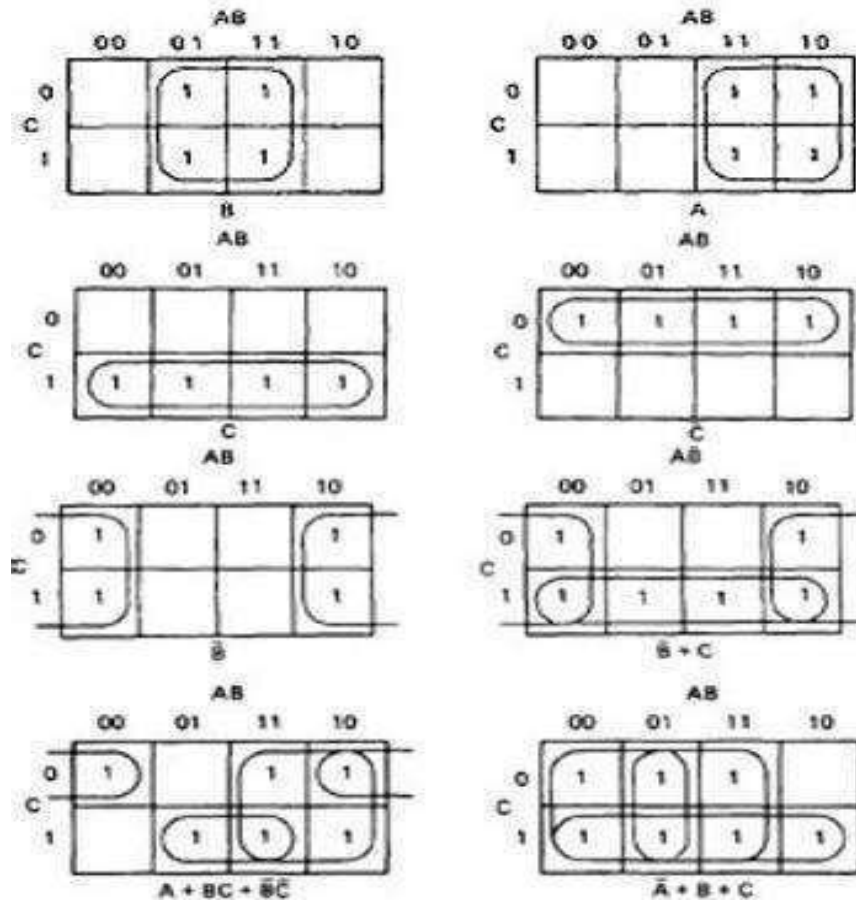
Figure 6.8: KV Charts for Functions of Three Variables.
