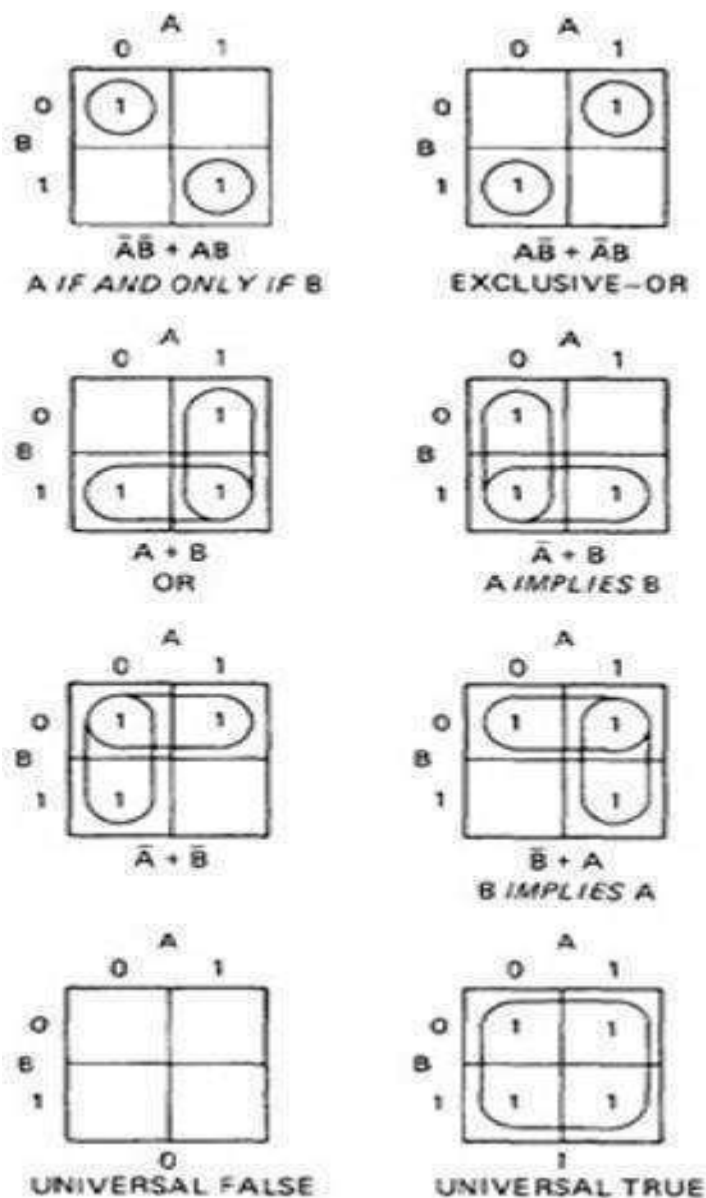
Figure 6.8: More Functions of Two Variables.
