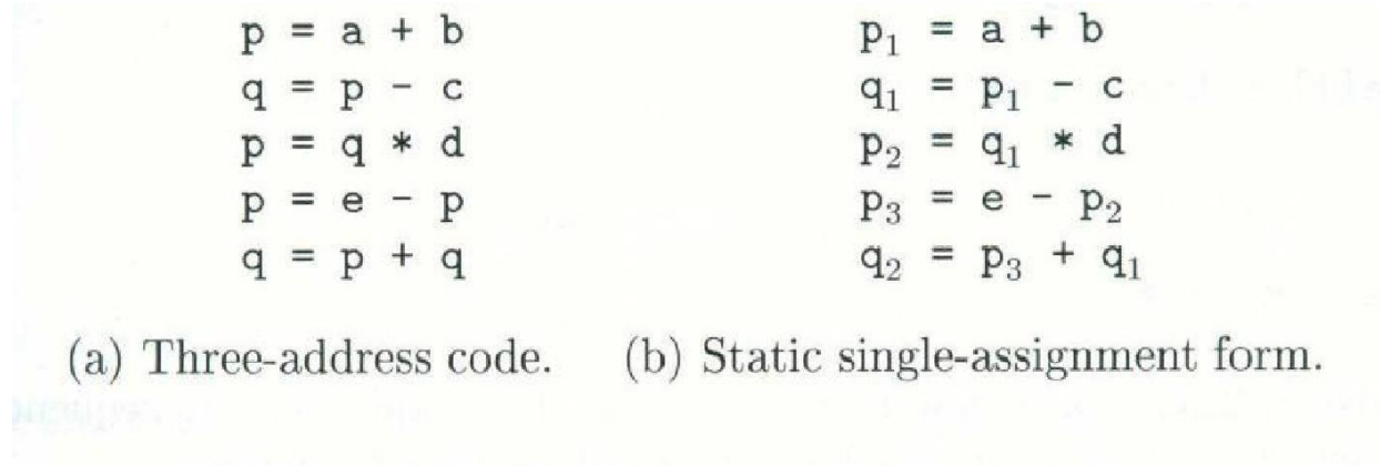
Figure 6.13: Intermediate program in three-address code and SSA
