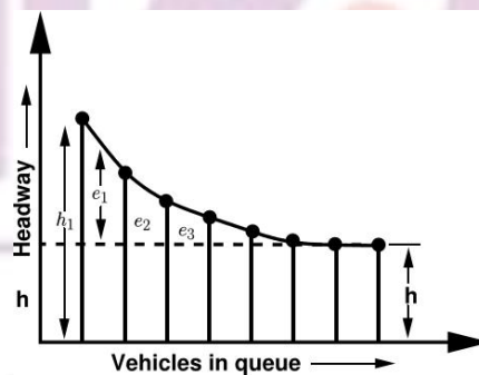
Fig.22 Headways departing signal
