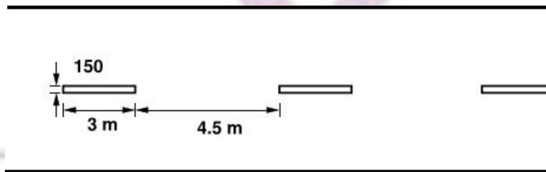
Fig.19 Centre line marking for a two lane road
