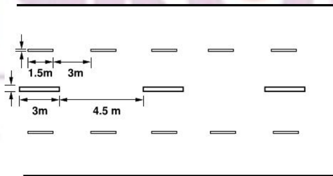
Fig.20 Centre line and lane marking for a four lane road
