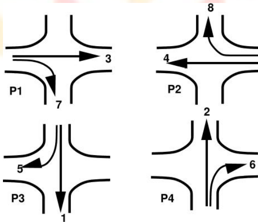
Fig. 21 One way of providing four phase signals
