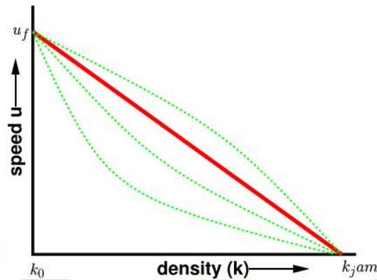
Fig.14 Speed-density diagram
