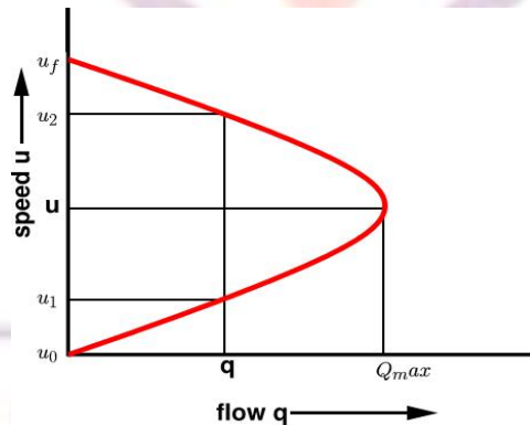
Fig.15 Speed-flow diagram
