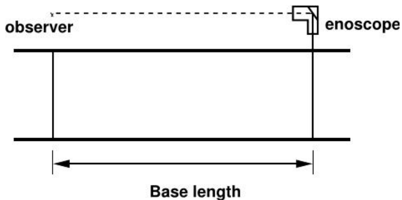
Fig. 16 Illustration of measurement over short section using enoscope
